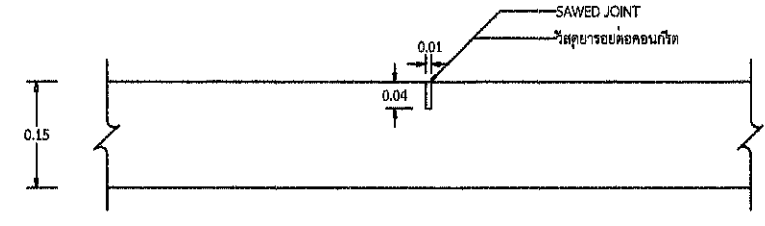
CONTRACTION JOINT NOT TO SCALE
