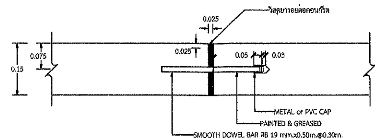
EXPANSION JOINT NOT TO SCALE
